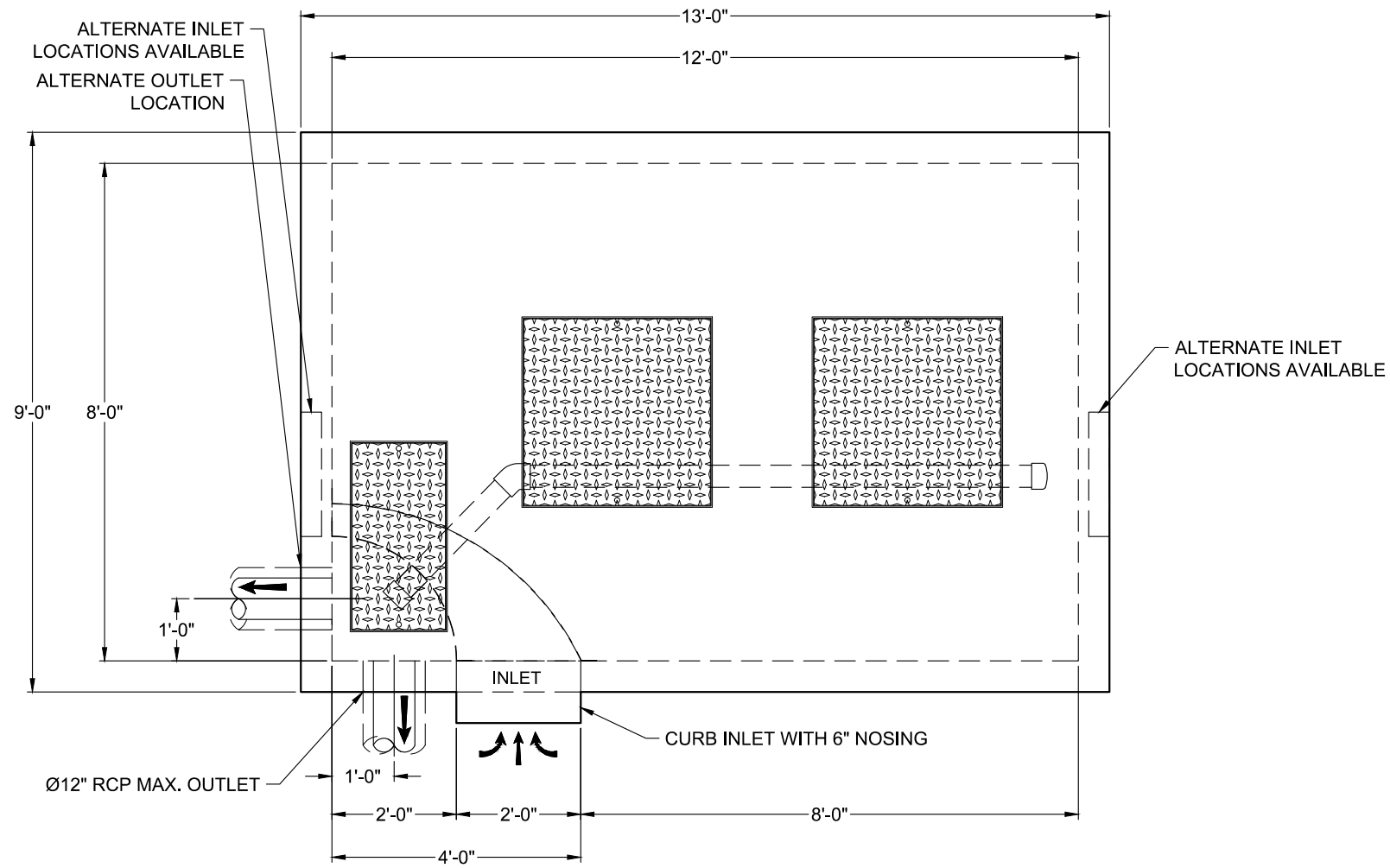
PLAN VIEW
