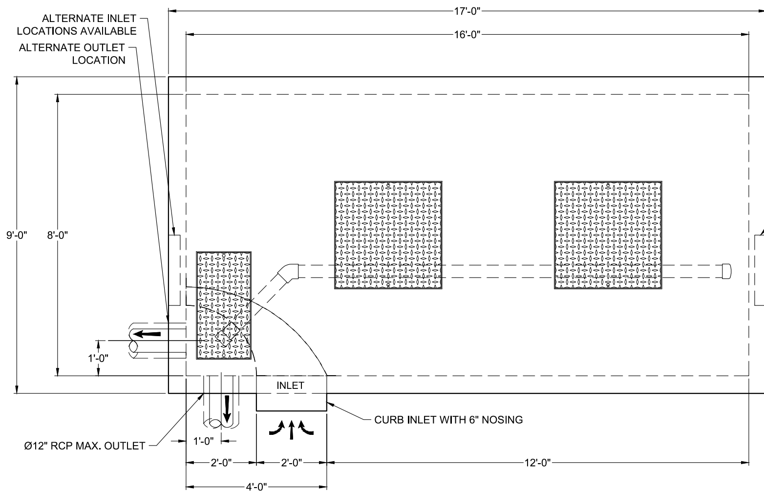
PLAN VIEW
