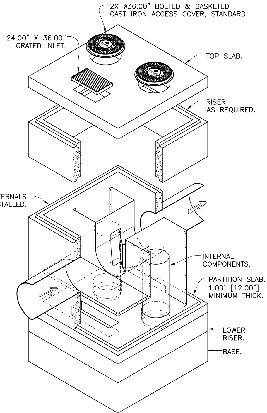
ISOMETRIC VIEW
