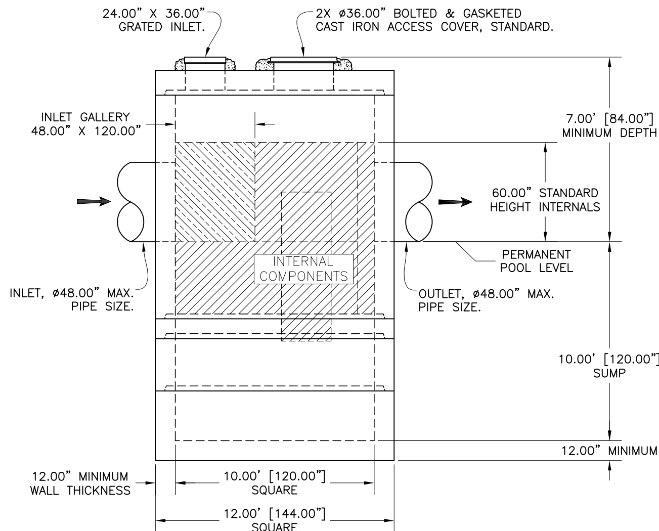
ELEVATION VIEW
