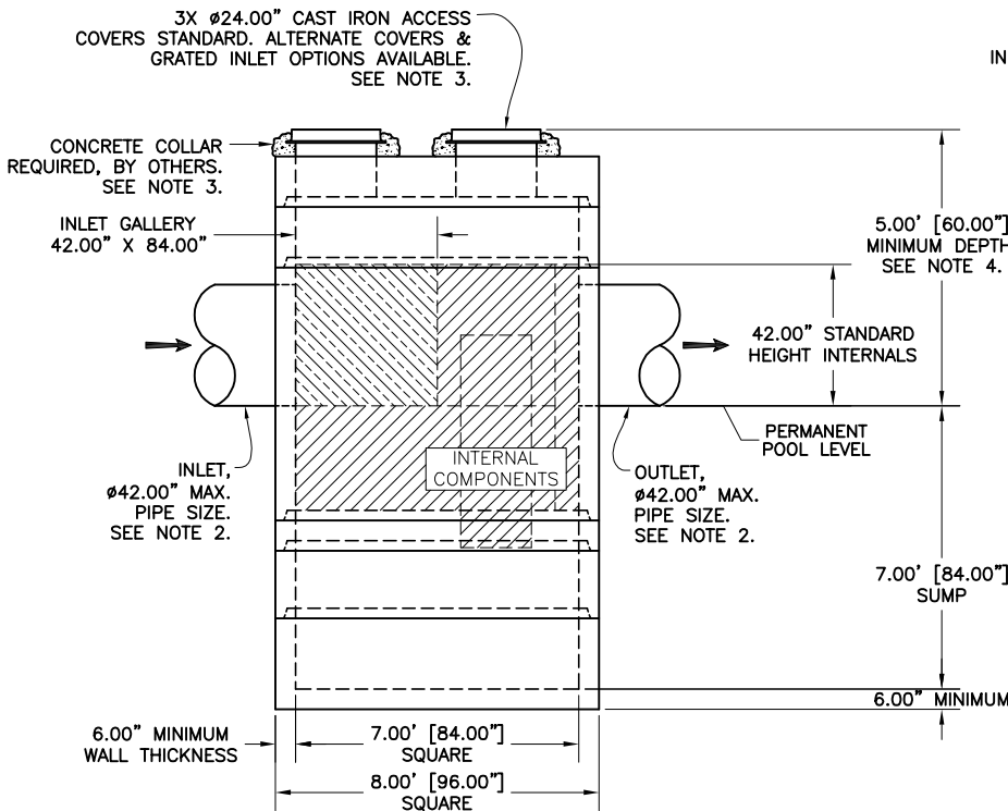
ELEVATION VIEW
