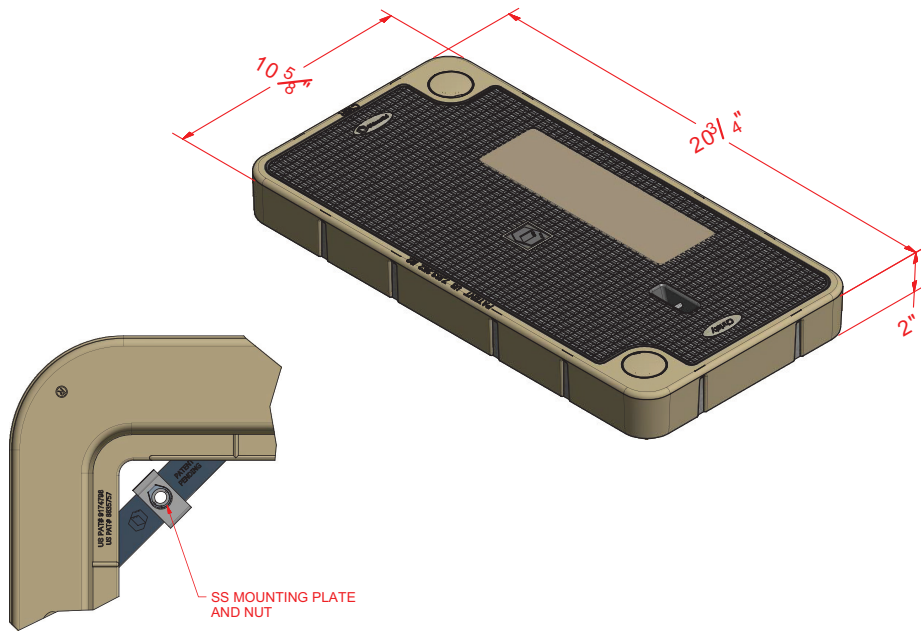
Bolt Down Detail
