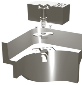
Bolt Down Detail
