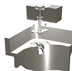
Bolt Down Detail
