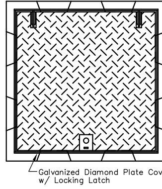
PLAN VIEW Shown With Cover
