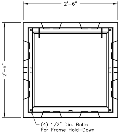
PLAN VIEW Cover Not Shown
