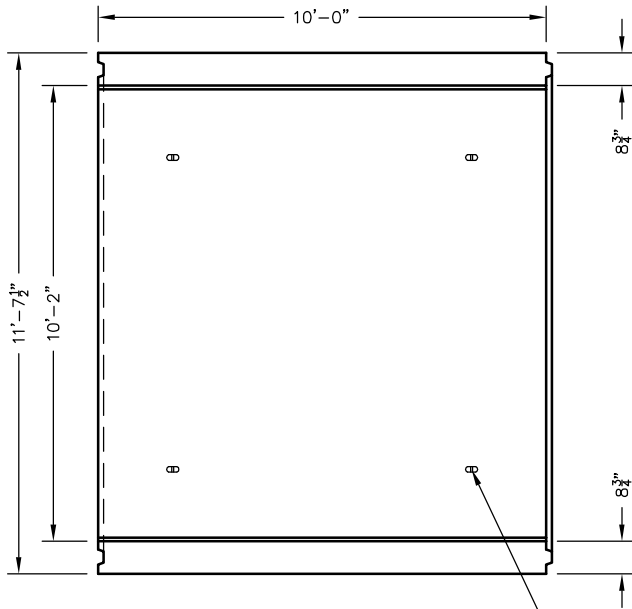
(4) - 8-Ton Lift Anchors PLAN VIEW - BASE
