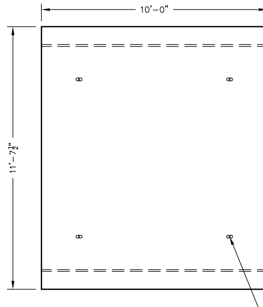
(4) - 8-Ton Lift Anchors PLAN VIEW - TOP
