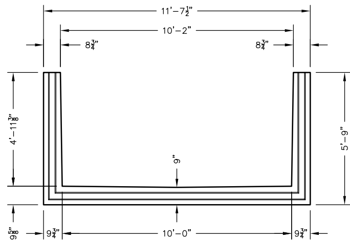
END VIEW - BASE
