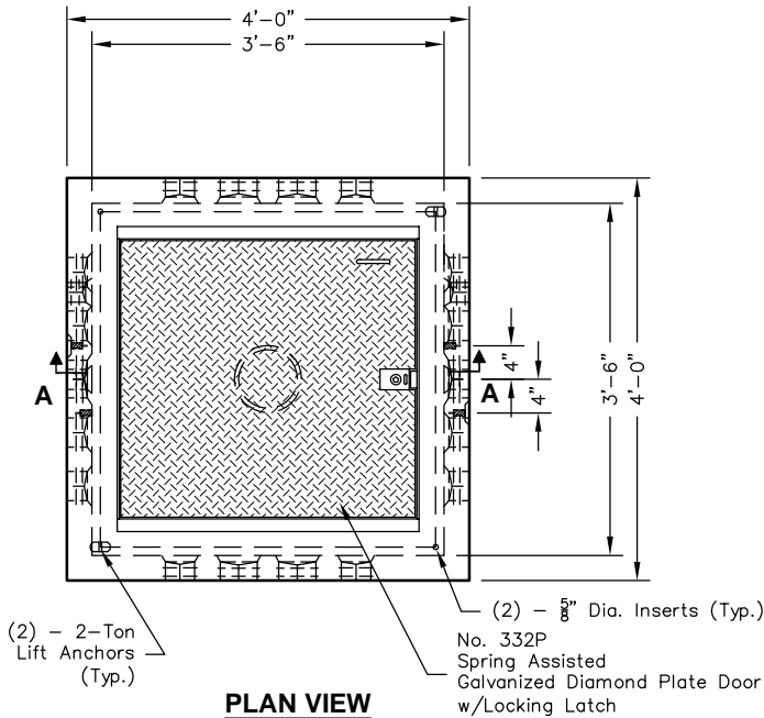
PLAN VIEW
