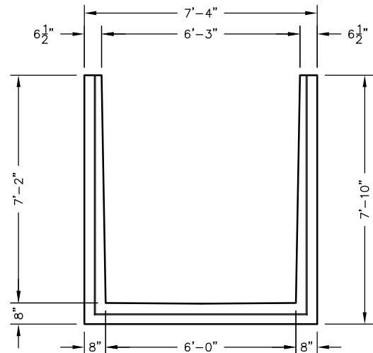
END VIEW - BASE
