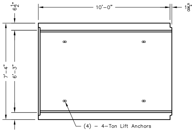
PLAN VIEW - BASE
