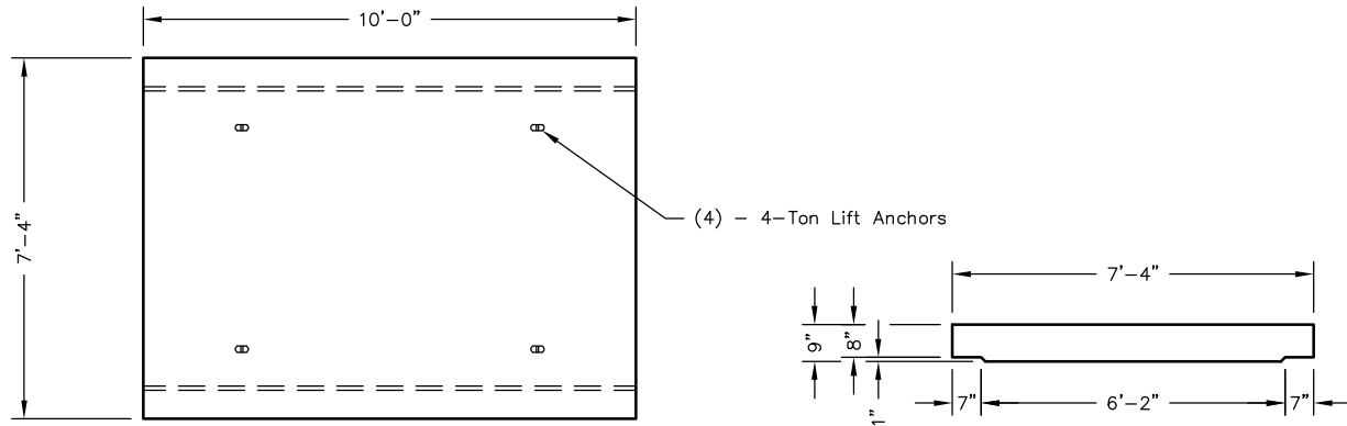
END VIEW - TOP
