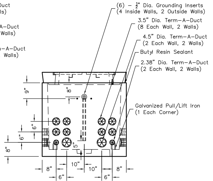
END VIEW
