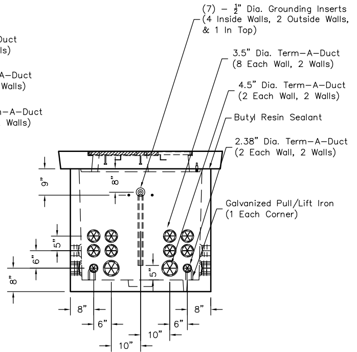
END VIEW
