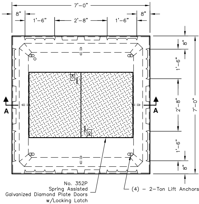
PLAN VIEW
