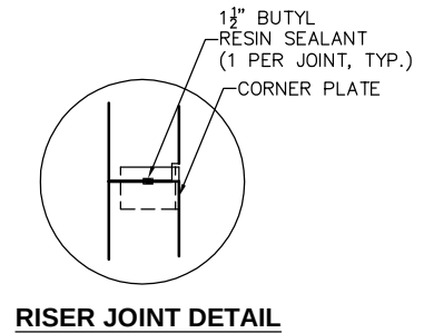
RISER JOINT DETAIL
