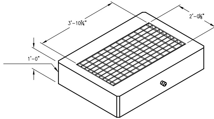
WSDOT TYPE 2 TOP 2,060 lbs.
