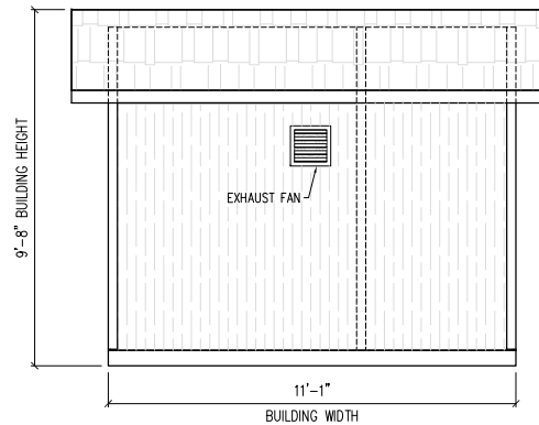
REAR ELEVATION
