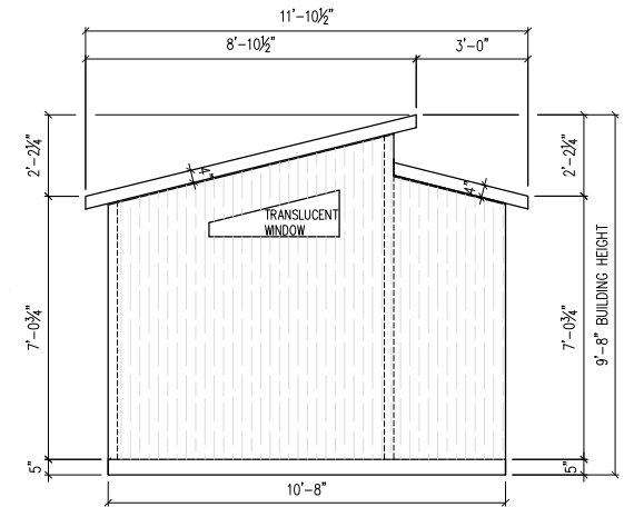
LEFT ELEVATION
