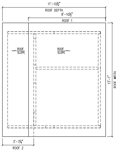
ROOF PLAN
