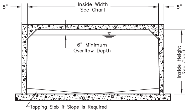
SECTION VIEW
