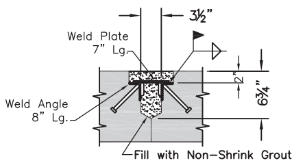
① Deck Joint Typical Between Top Sections & Flat Slab Base Sections
