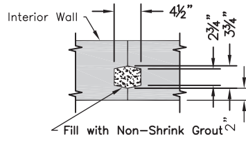
② Vertical Wall Joint Typical Between Top Sections
