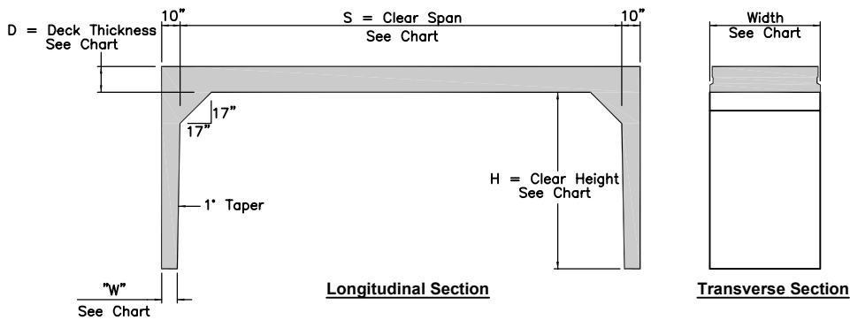
Sizing And Weights (KIPS) for Standard Product
