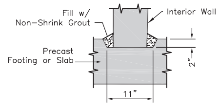
③ Footing Keyway
