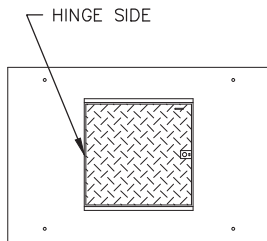
LOCKING STEEL COVER No. 57TL-332P 3,000 lbs.
