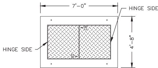
LOCKING STEEL COVERS No. 57TL-2-332P 2,250 lbs. PSE Code #7663200 (Base and Cover Assembly)
