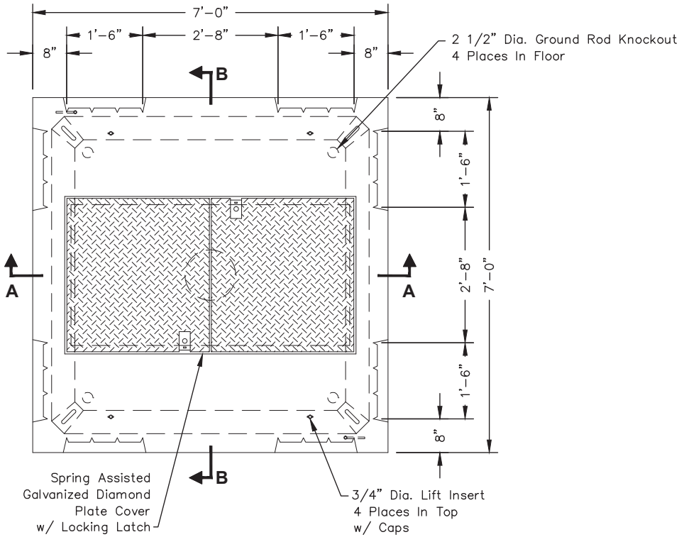
PLAN VIEW
