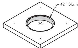
ROUND ACCESS OPENING No. 77-42C 4,150 lbs
