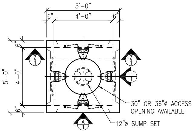
PLAN VIEW SCALE: 1/4" = 1'-0"
