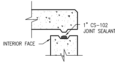
TOP SLAB WITH TONGUE & GROOVE JOINT N.T.S.
