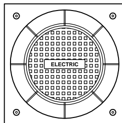
with 30"φ Ring and Cover
