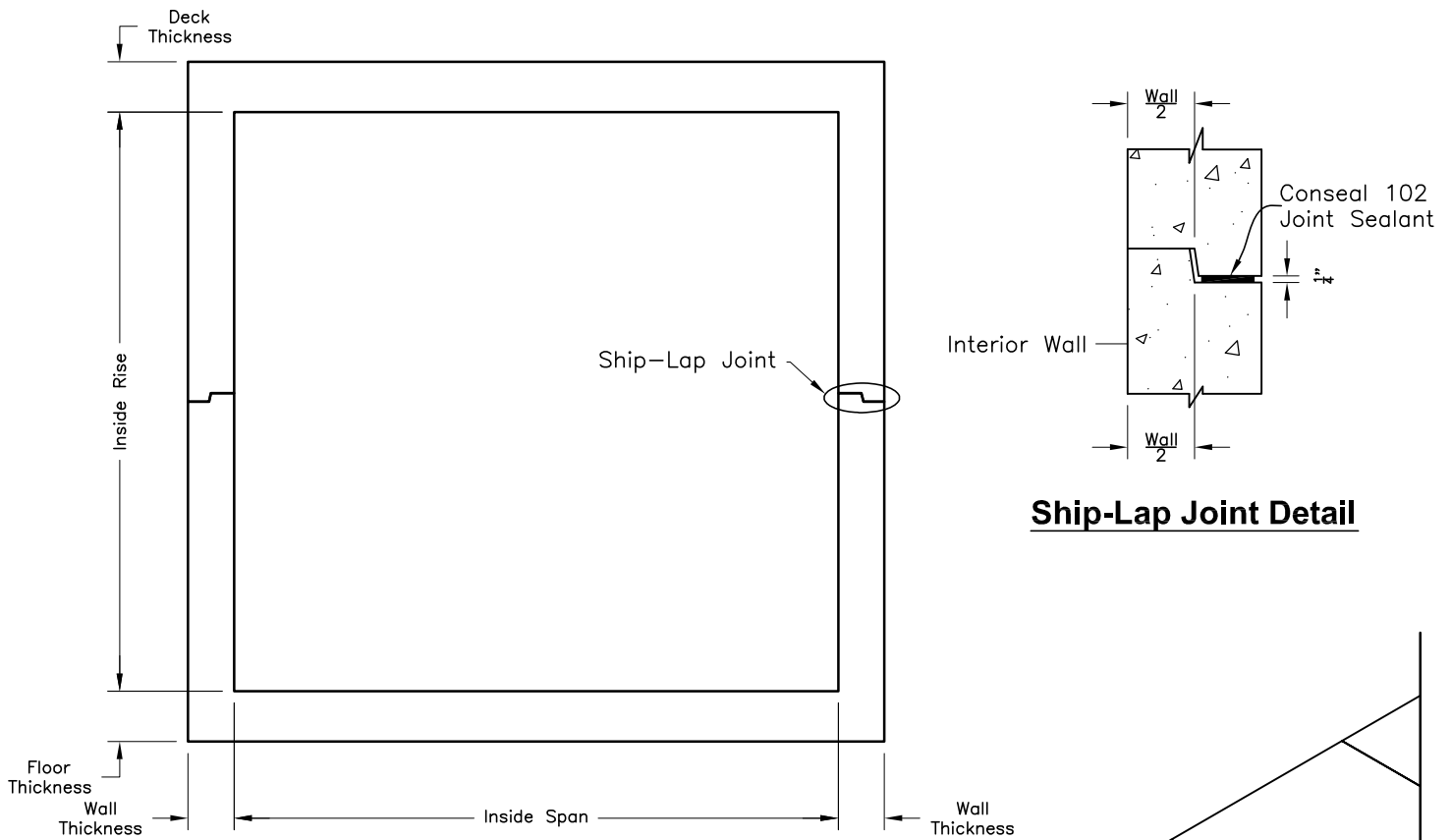
Culvert Cross Section
