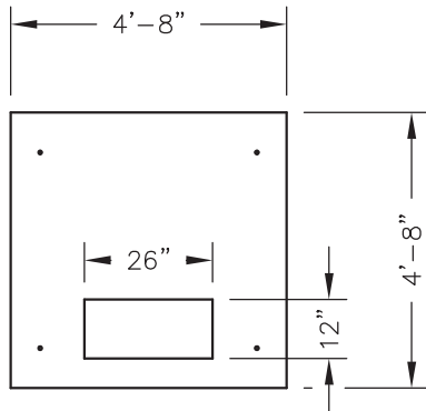
PADMOUNT No. 55-1226 1,550 lbs.
