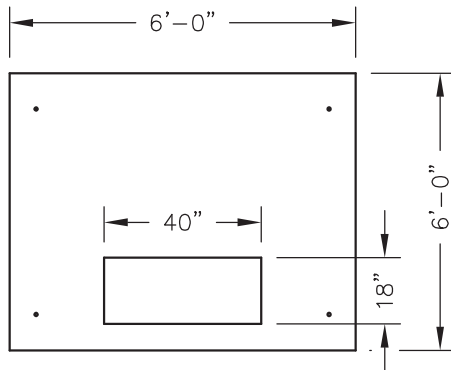
PADMOUNT No. 66-1840 2,300 lbs.
