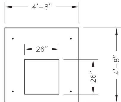
PADMOUNT No. 55-2626 1,400 lbs.
