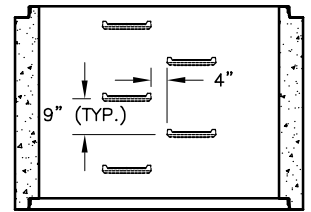
Manhole Step Detail
