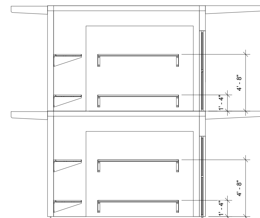
3 END WALL BUNK LOCATIONS 1/4" = 1'-0"
