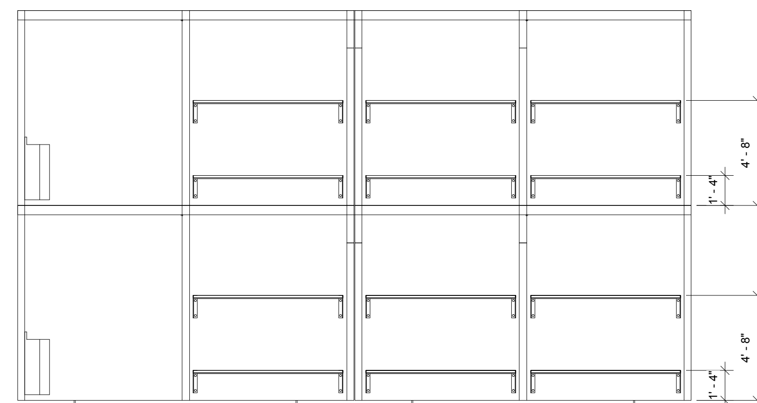
2 BACK WALL BUNK LOCATIONS 1/4" = 1'-0"
