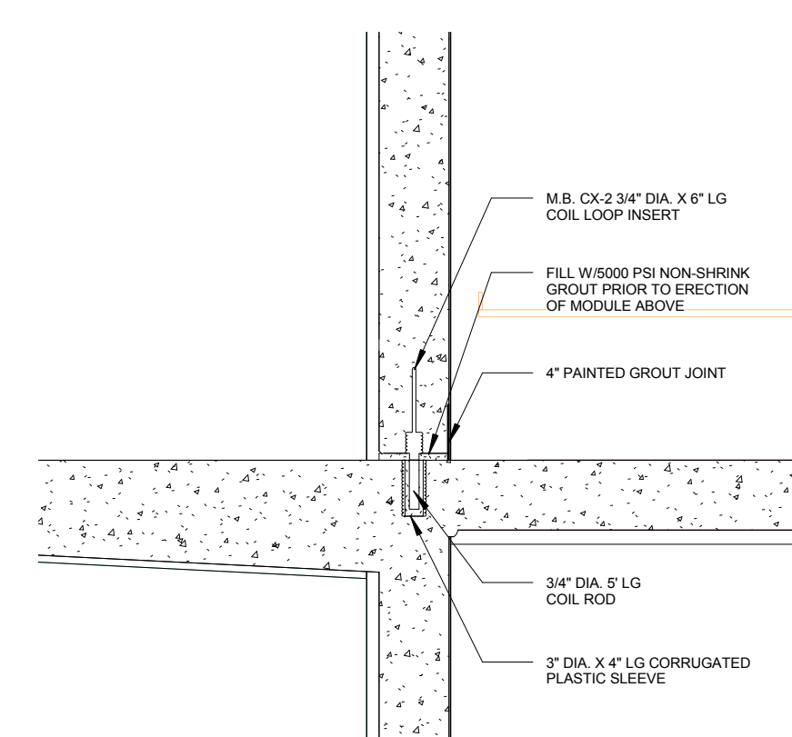
6 CELL TO CELL CHASE SIDE 1" = 1'-0"
