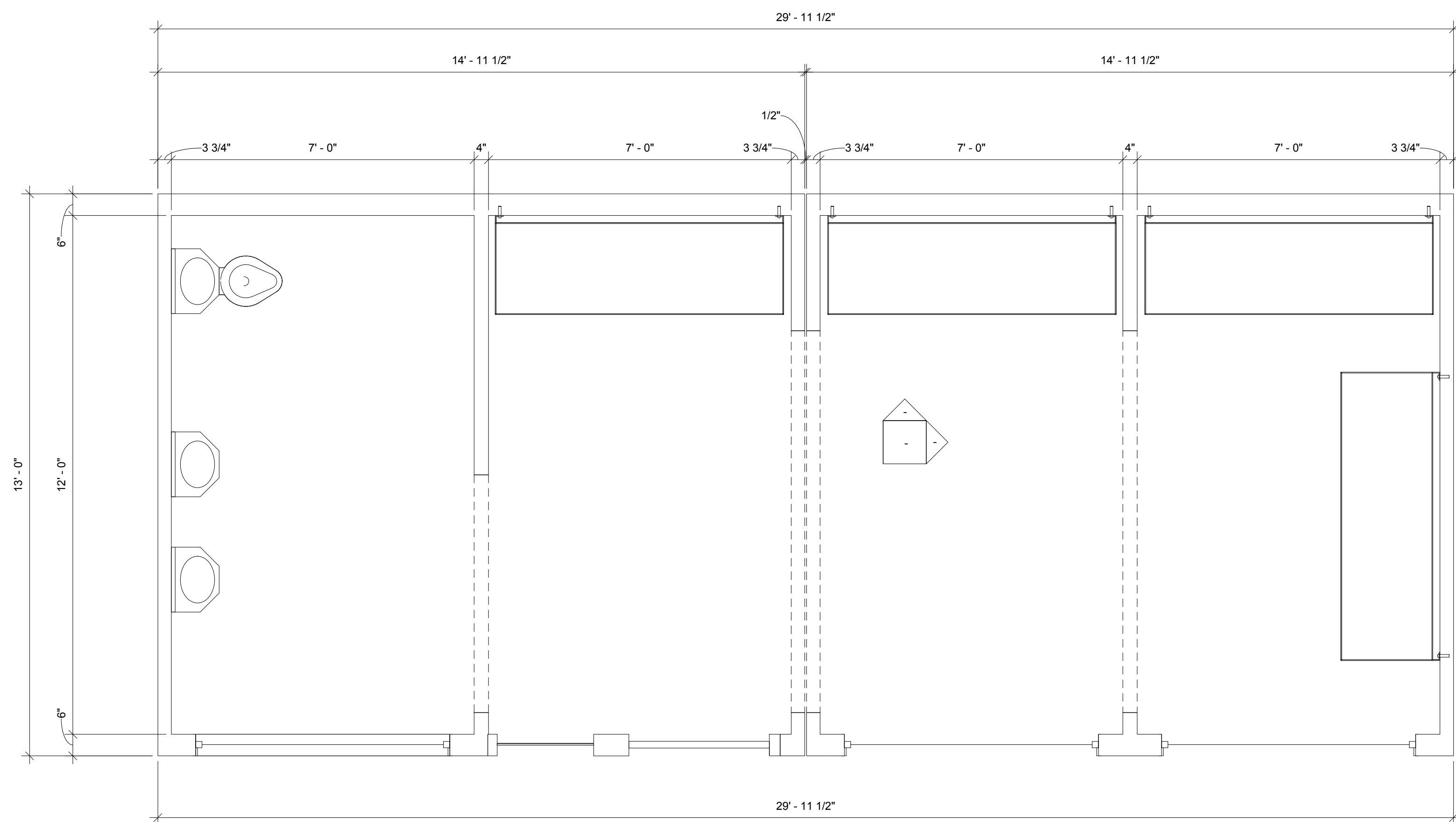
1 PLAN VIEW 1/2" = 1'-0"
