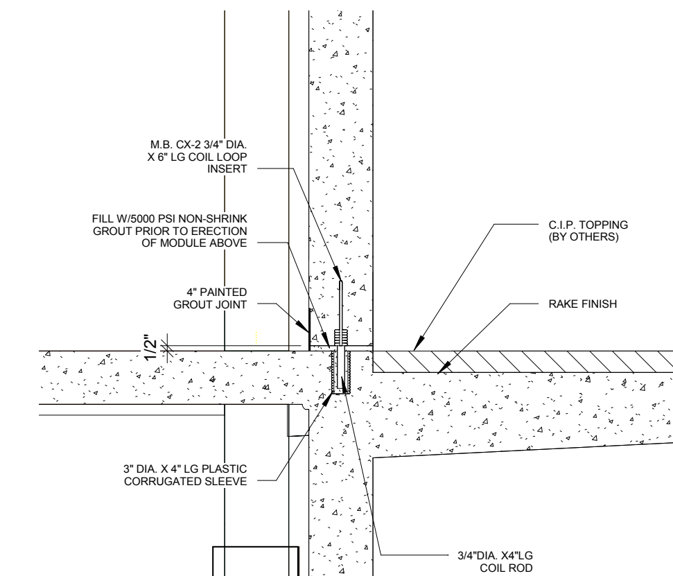
5 CELL TO CELL CONNECTION 1" = 1'-0"
