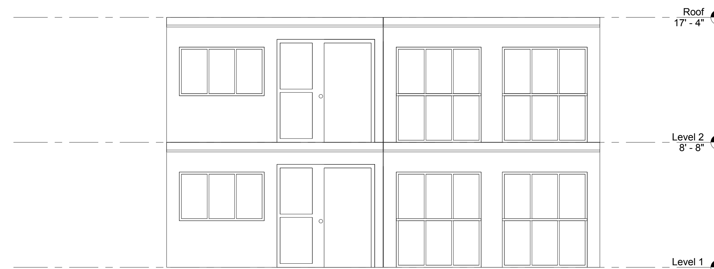
4 DOOR AND WINDOW LOCATIONS 1/4" = 1'-0"
