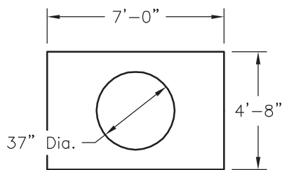
Concrete w/Hole No. 57-T37C 3,350 lbs.
