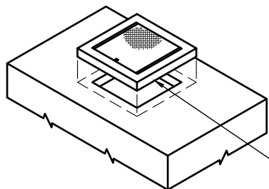
Locking Steel Cover No. 44-332P 835lbs.
