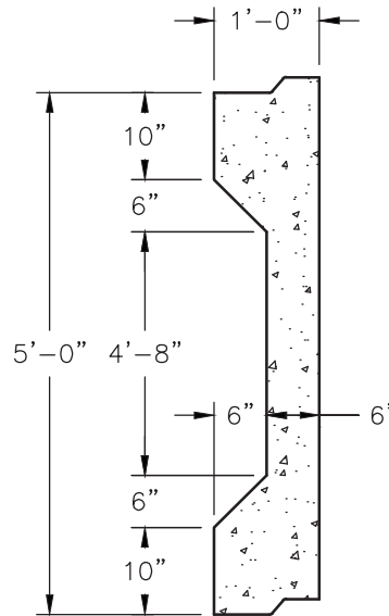
SECTION AT SIDES
