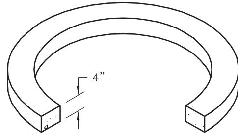
NO. GR3704 37" Inside diameter 48" Outside diameter 260 lbs.
