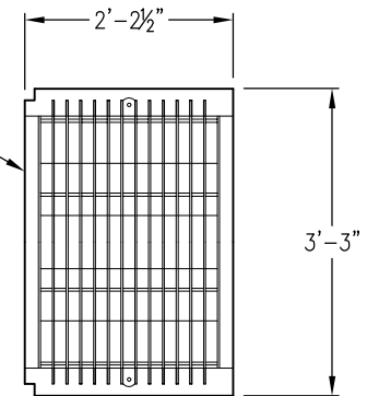
GALVANIZED STEEL FRAME AND GRATE, SEE NOTE 1.
