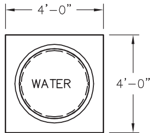
Cast Iron Frame And Cover No. 44-32CI 1500 lbs.
