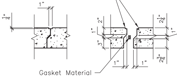
Section View Of Trench Keyway
