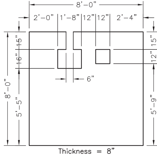
8' x 8' SM-637162 (750 through 1000 KVA) 4,560 Lbs.
