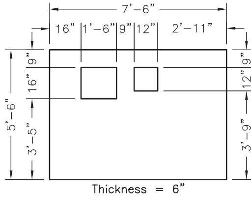
66 x 90 SM-637160 (0 through 500 KVA) 2,870 Lbs.
