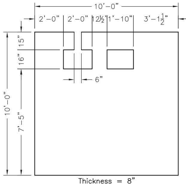
10' x 10' SM-637163 (1500 through 2500 KVA)
