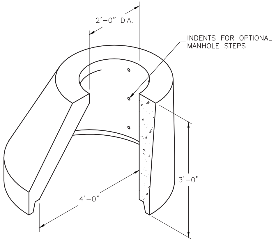
48" X 24" MANHOLE ECCENTRIC CONE
