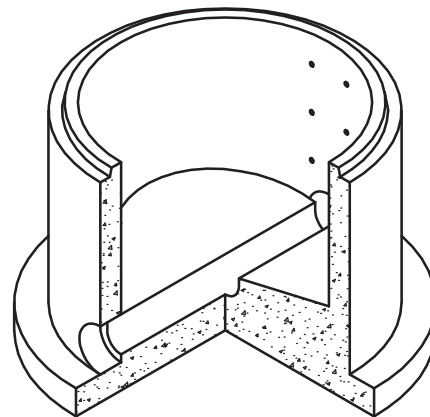
48" BASE WITH INVERT AND ANTI FLOATATION
