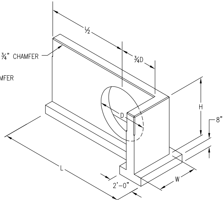
RIGHT HAND HEADWALL
