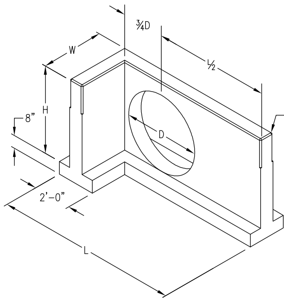
LEFT HAND HEADWALL
