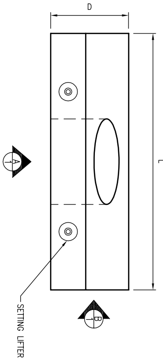
PLAN VIEW SCALE: 1/2" = 1'-0"
