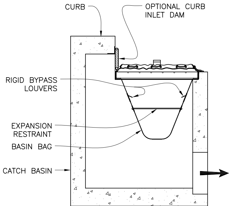
SECTION VIEW -INSTALLED- WITH OPTIONAL CURB INLET DAM
