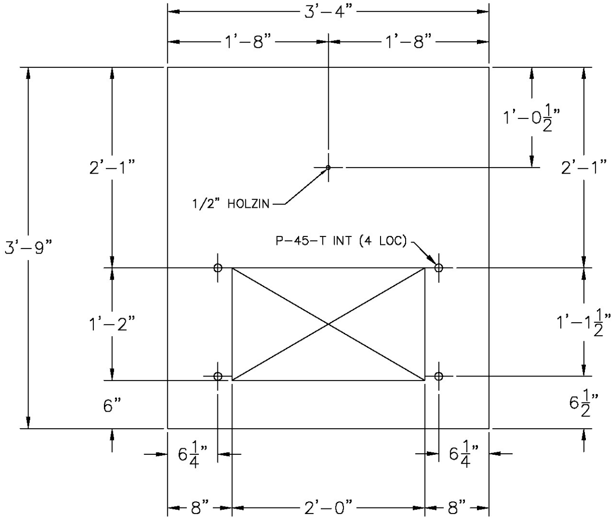
PLAN VIEW
