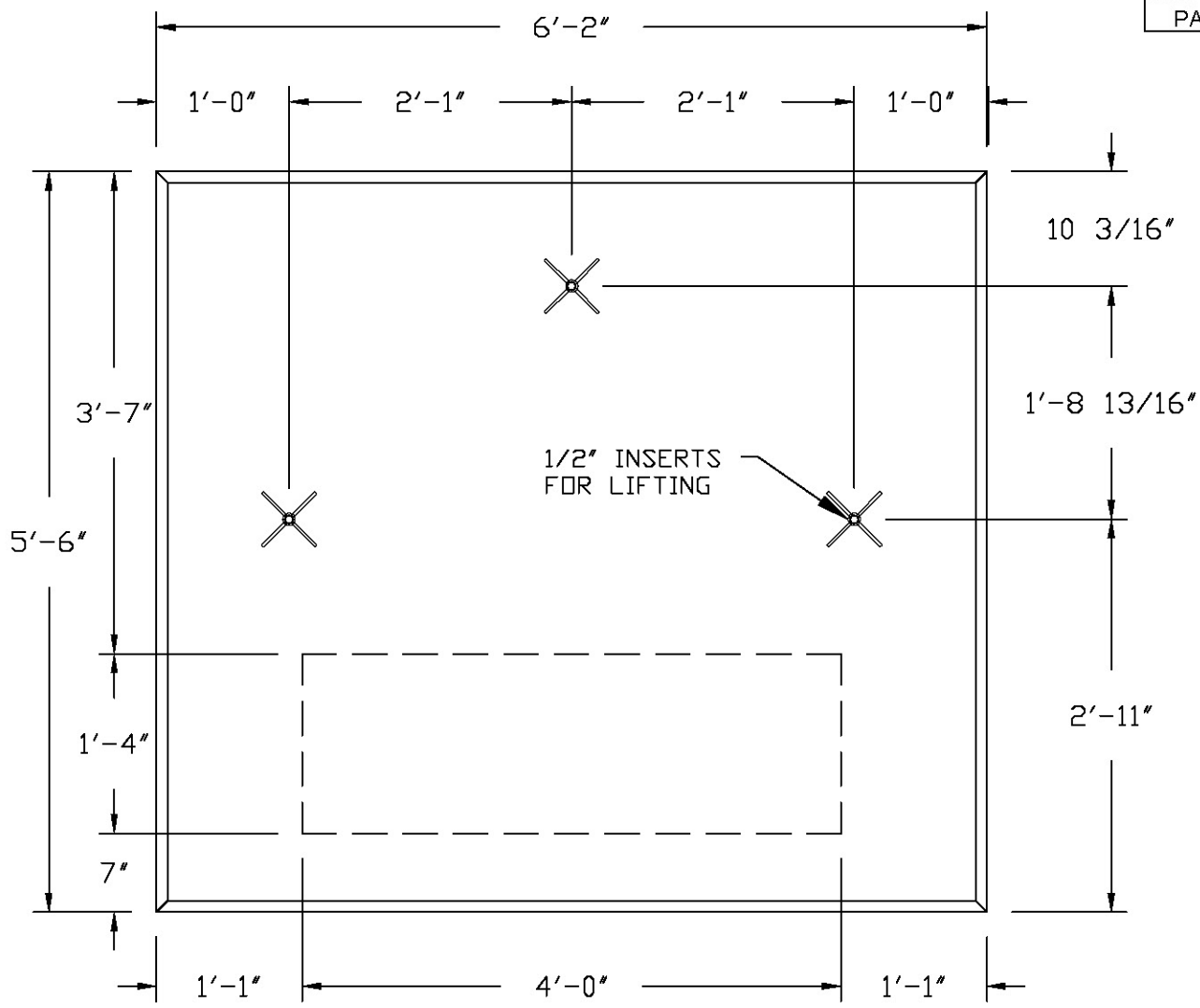
PLAN VIEW
