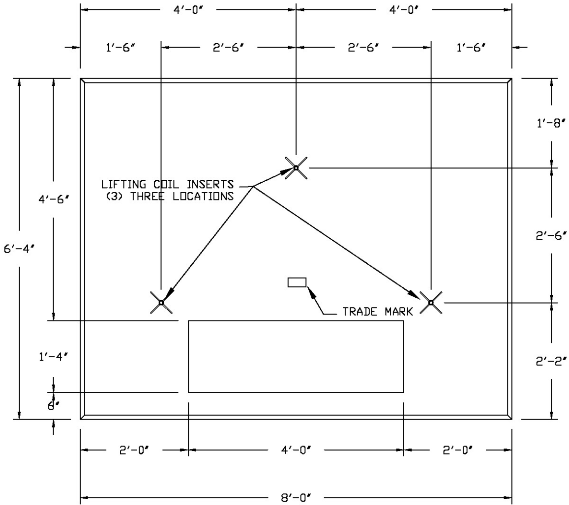
PLAN VIEW
