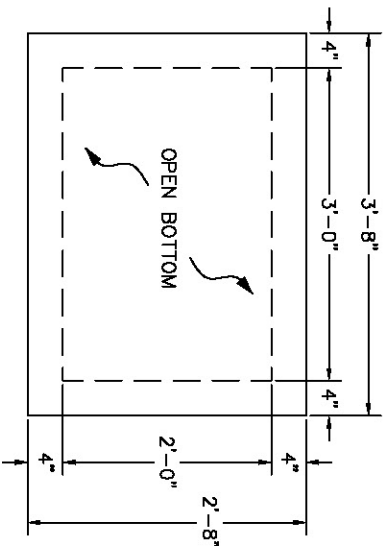
PLAN VIEW
