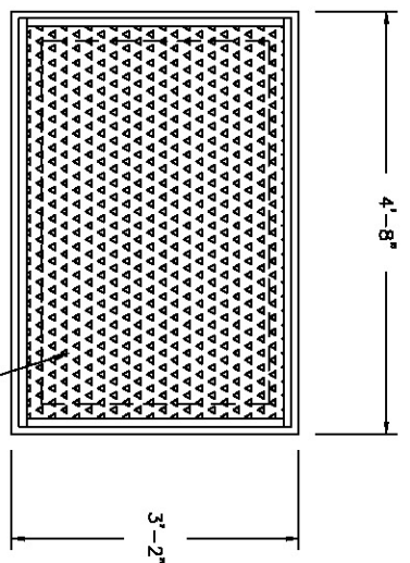
FRAME AND COVER DETAIL
