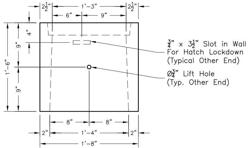
Pull Box End View
