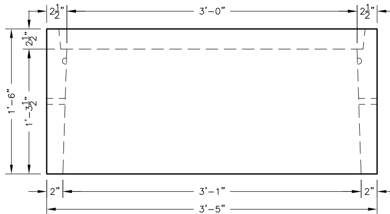
Pull Box Side View
