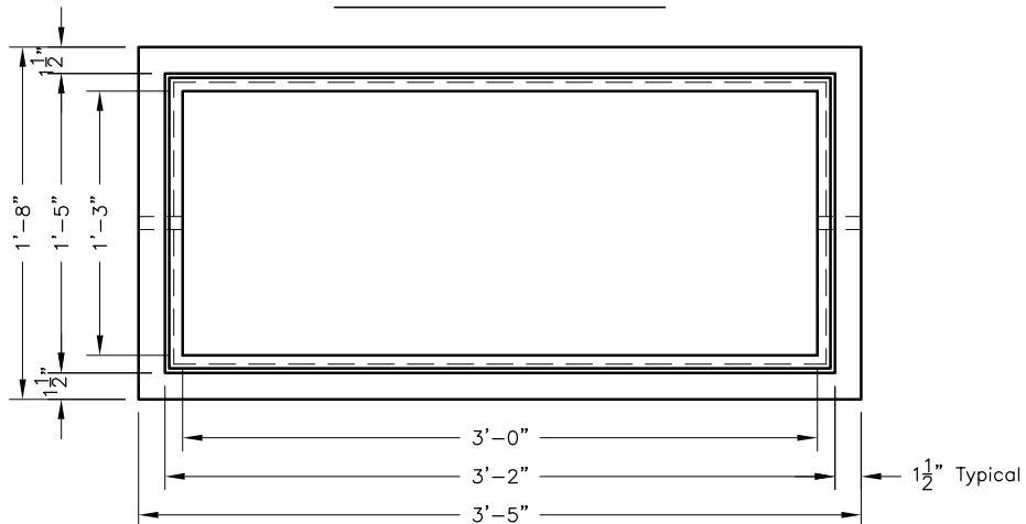
Pull Box Plan View
