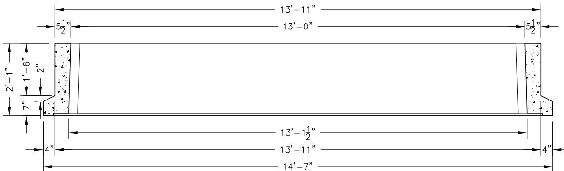
Pit Section B
