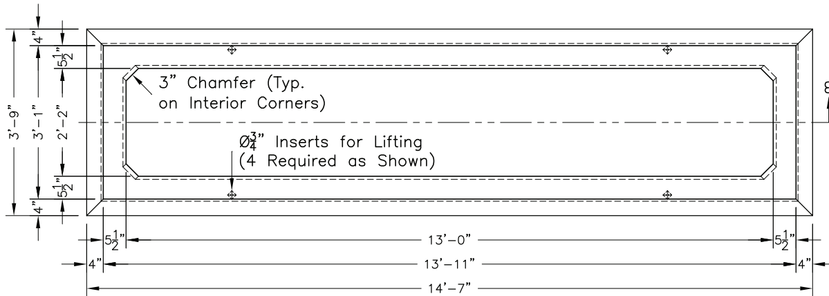
Pit Plan View
