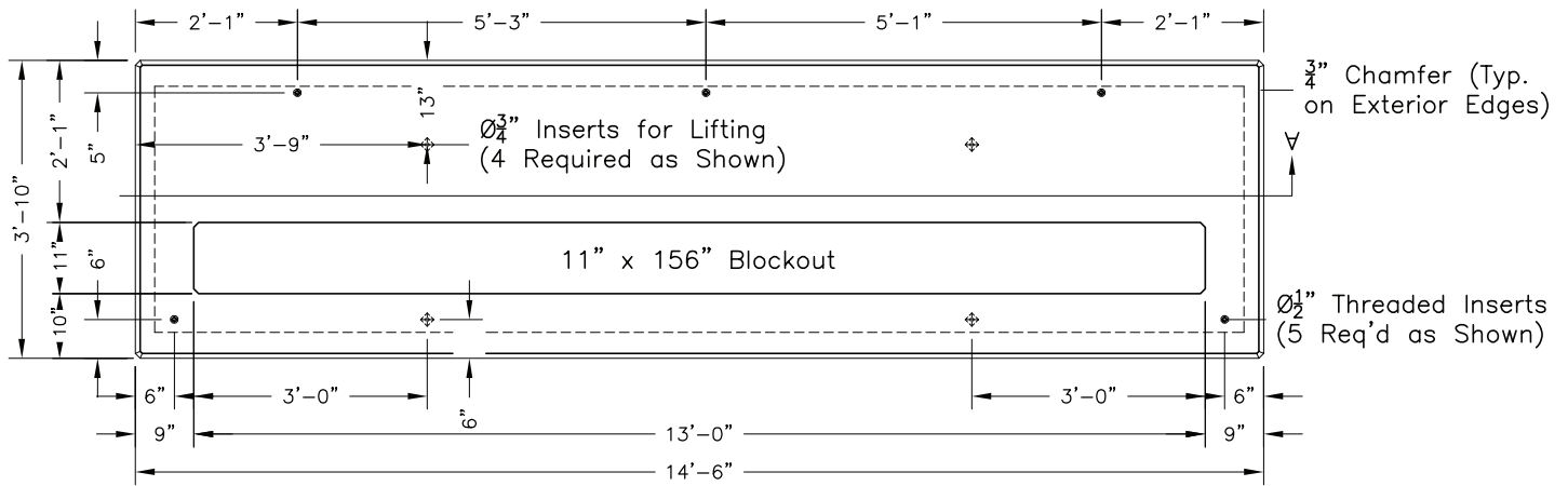
Pad Plan View
