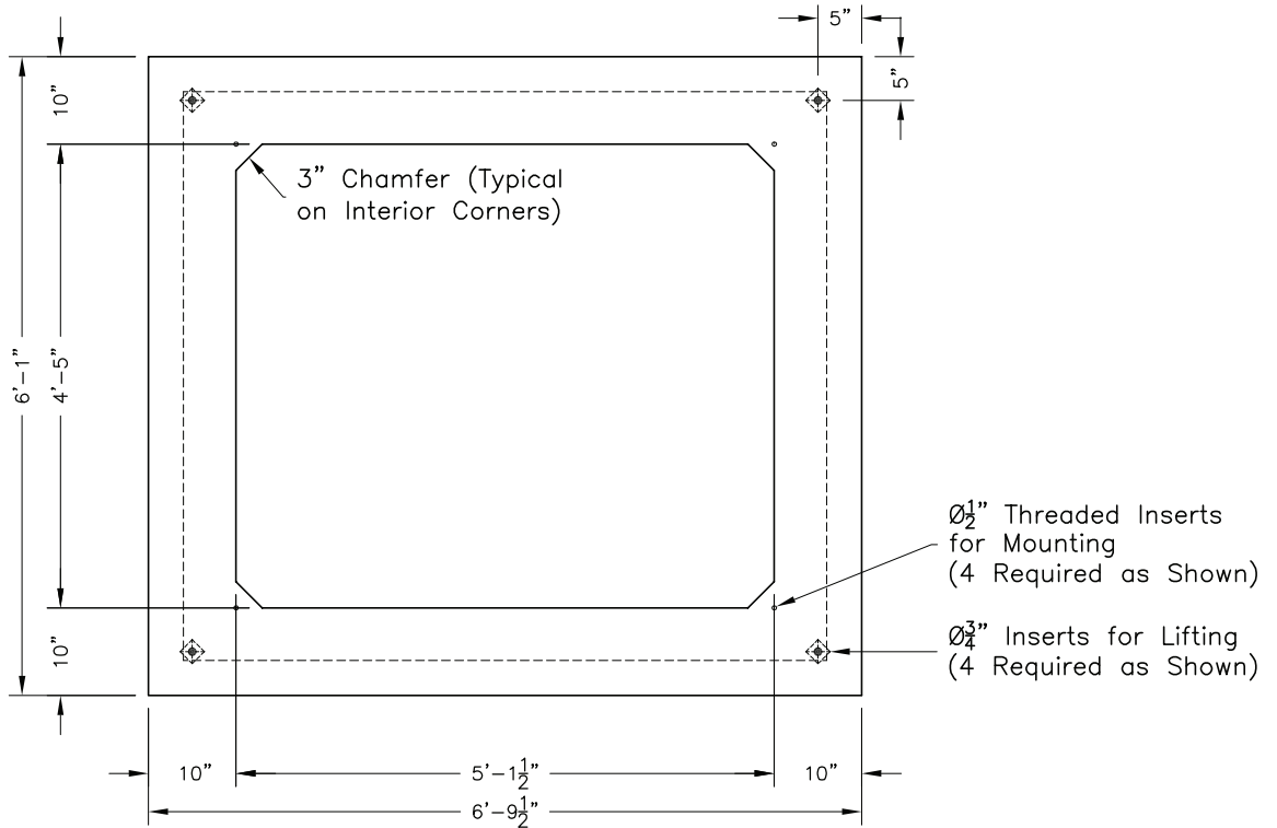
Plan View
