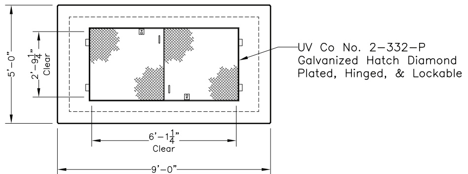
Lid Plan View
