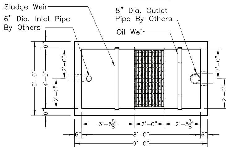
Base Plan View
